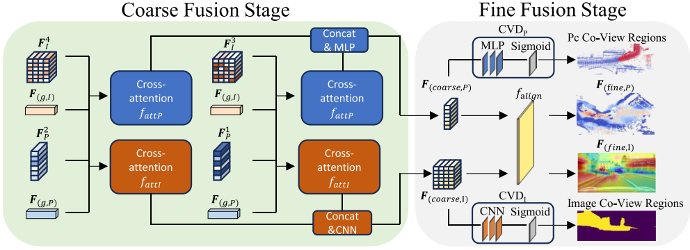
Fig. 3. The overall architecture of SFAM. SFAM fuses image and point cloud features in a coarse-to-fine manner. In the coarse fusion stage, symmetric cross-attention is leveraged to fuse multi-scale image and point cloud features. In the fine-grained fusion stage, fine-grained features F_{(fine,P)} and F_{(fine,I)} are extracted by a weight-sharing network f_{align} . In addition, coarse-grained features F_{(coarse,P)} and F_{(coarse,I)} are used as inputs of the CVD, where CVD_I is the image CVD and CVD_P is the point cloud CVD.
