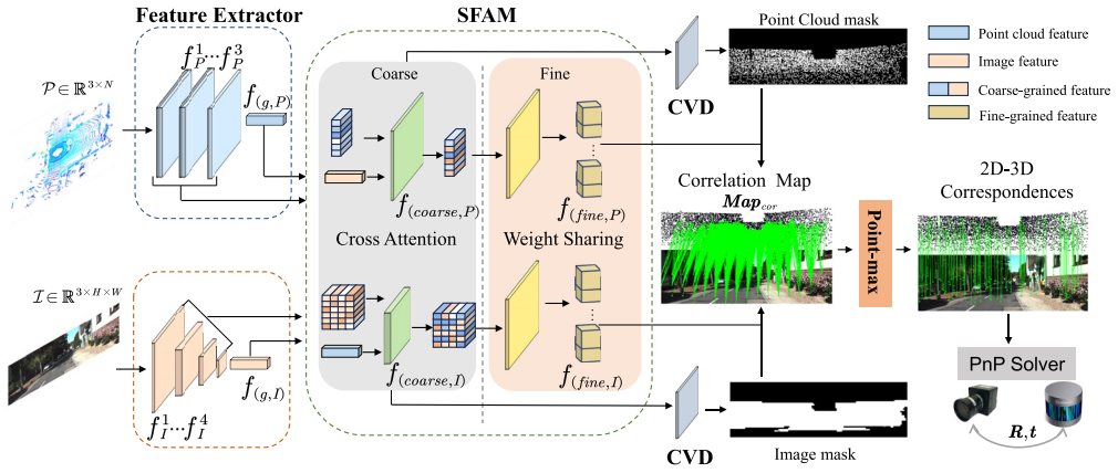
Fig. 2. Overview of I2P ppsim . I2P ppsim is composed of five modules: Feature Extractor, SFAM, CVD, point-max, and PnP solver. Firstly, the high-dimensional features of images and point clouds are separately extracted by the two branches of Feature Extractor. Such features are then fed into SFAM to obtain cross-modal features in a coarse-to-fine architecture. With the coarse-grained features from SFAM, the co-view region of the image and point cloud is determined by CVD. Further, based on the fine-grained features from SFAM and the outputs of CVD, a correlation map is predicted, where 2D-3D correspondences are selected by point-max. At last, the relative pose of the LiDAR to the camera is estimated via the PnP solver. CVD, co-view detector; PnP, perspective-n-point.
