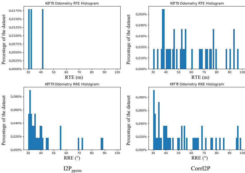
Fig. 7. Histograms of error distributions of I2P ppsim and CorrI2P at high RTE and RRE thresholds.
