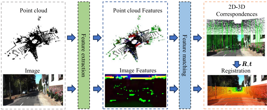
Fig. 1. The general pipeline of image-to-point cloud (I2P) registration. I2P registration first extracts the common features and then conducts the feature matching to build the 2D-3D correspondences. After that, a perspective-n-point (PnP) solver is used to estimate the relative pose.
